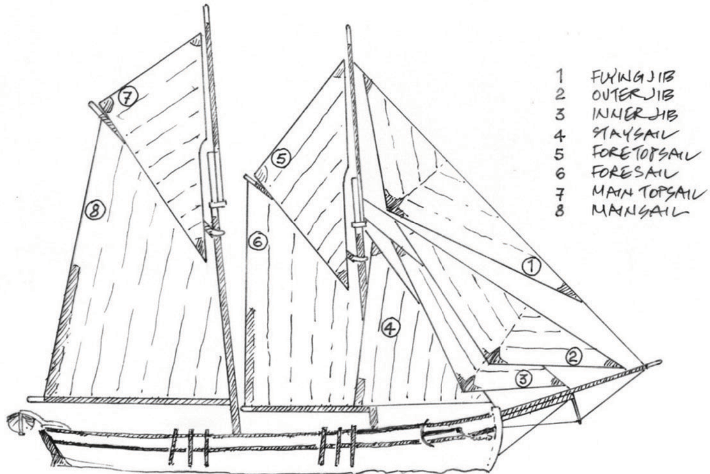
SCHOONER "LA BOHÈME" SAIL PLAN Emile de Beauville 7/14
